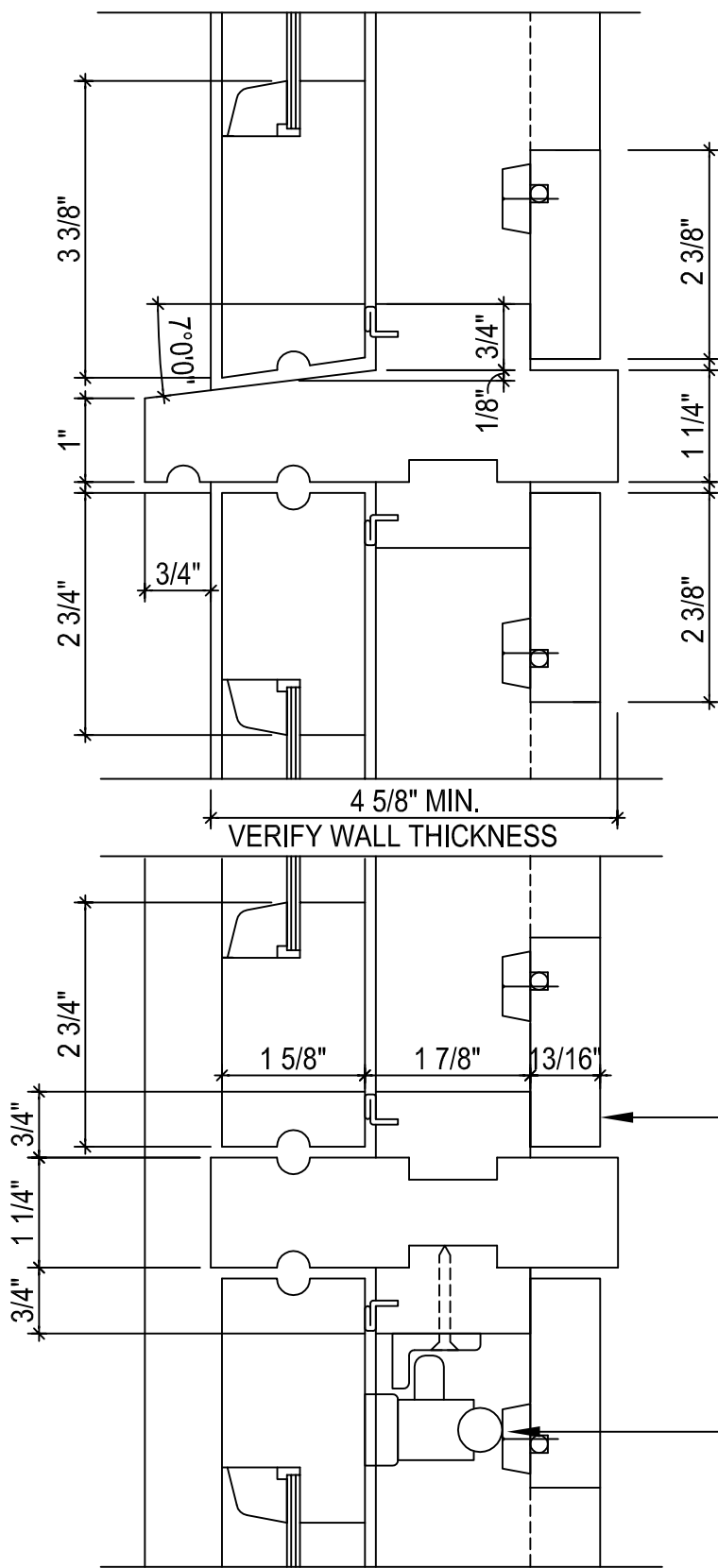
F HORIZONTAL MULLION
